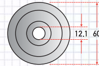
Single bolthole add to code: BH12
