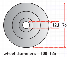
Single bolthole
